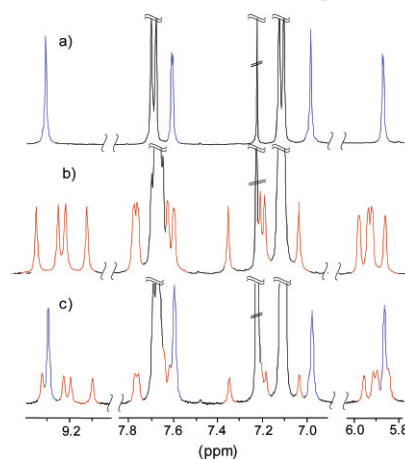
Fig. 1 Sections of the 1 H NMR (400 MHz, CDCl 3 , 25 °C) spectra of: a) homodimer 1-1 ; b) homodimer 3-3 ; c) mixture of 1 and 3 resulting in two homodimers.
