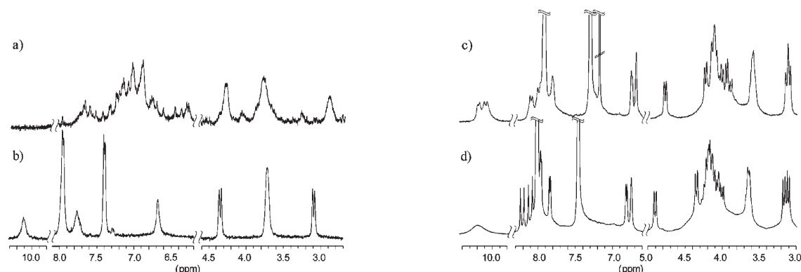
Fig. 2 Selected 1 H NMR spectra (400 MHz, 25 °C) of tetraureas: a) irregular aggregates of 1 in CD 2 Cl 2 ; b) homodimer 2-2 in CD 2 Cl 2 ; c) homodimer 4-4 in CDCl 3 ; d) homodimer 4-4 in CD 2 Cl 2 .
